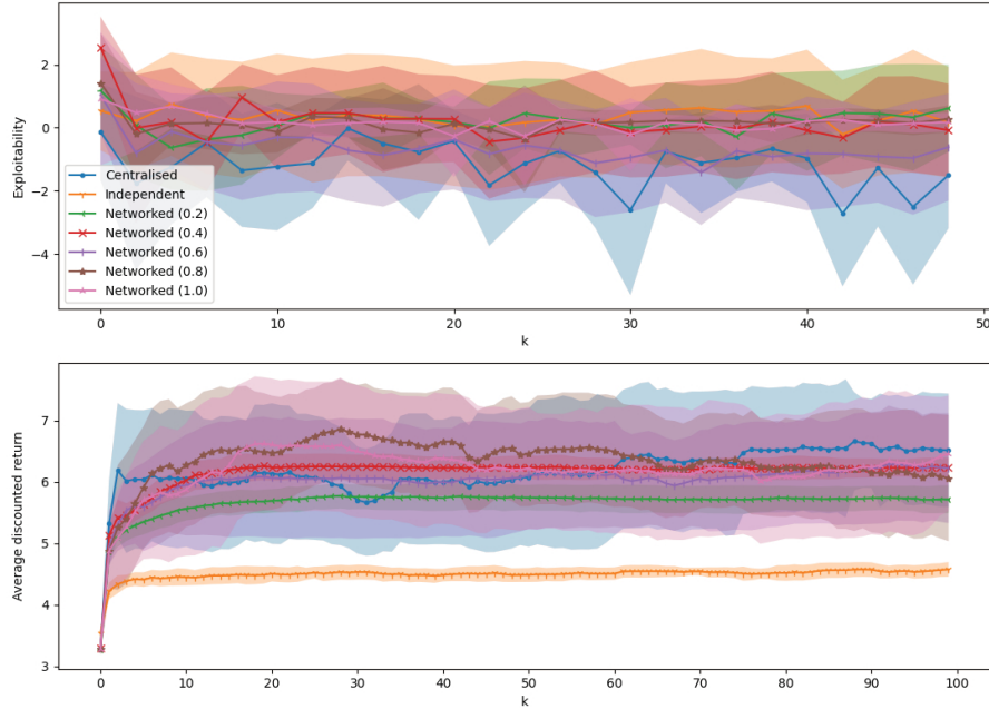
Fig. 7. ‘Evade’ task, population-dependent policies with estimated mean-field distribution, 10x10 grid.
