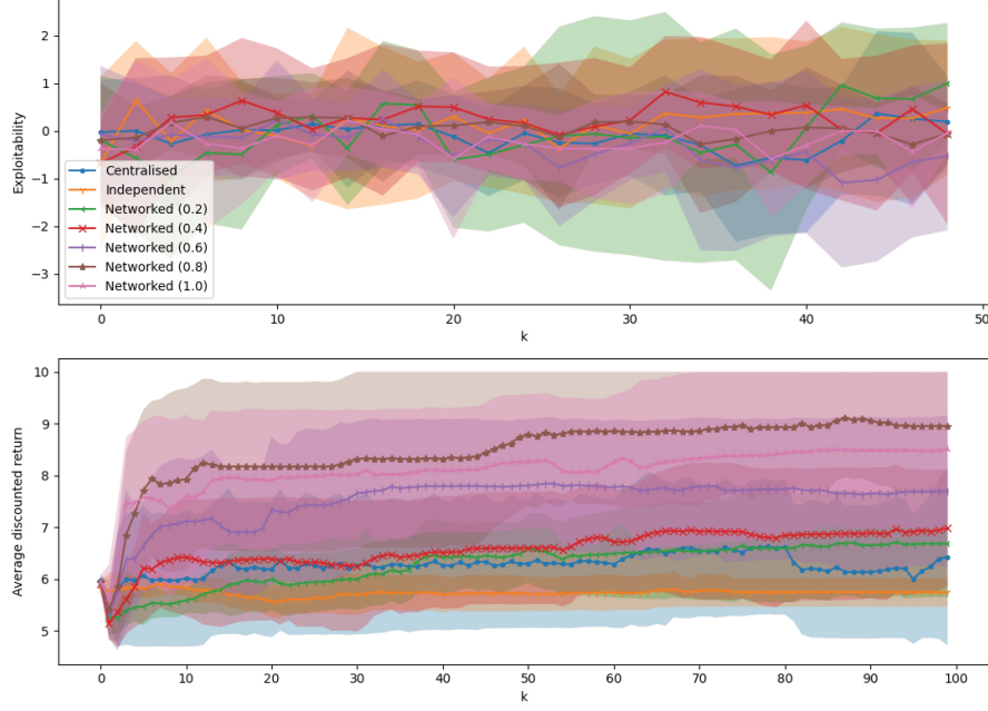
Fig. 6. ‘Push object’ task, population-dependent policies with estimated mean-field distribution, 10x10 grid.
