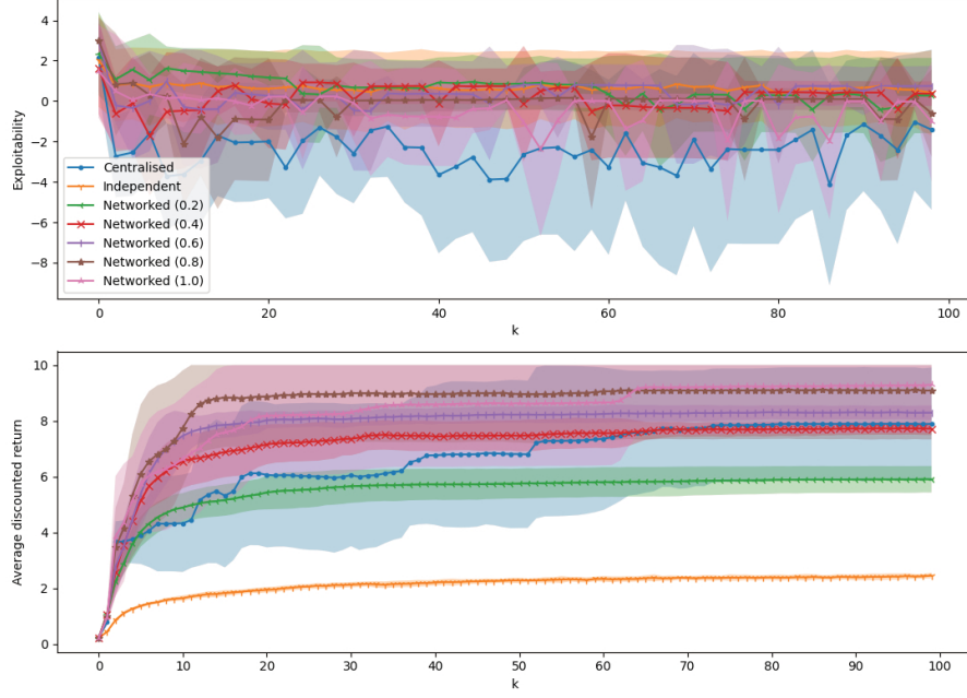
Fig. 4. ‘Cluster’ task, population-independent policies, 50x50 grid.
