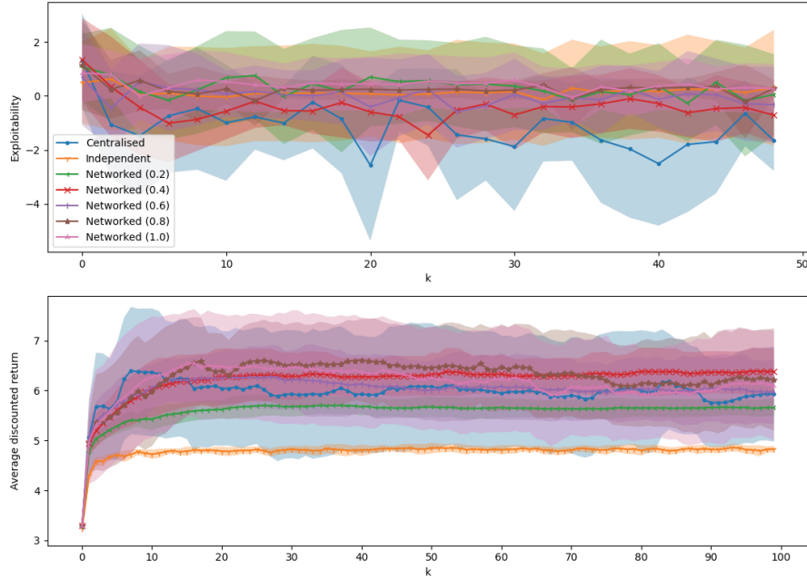
Fig. 9. ‘Evade’ task, population-dependent policies with global observability of mean field, 10x10 grid.
