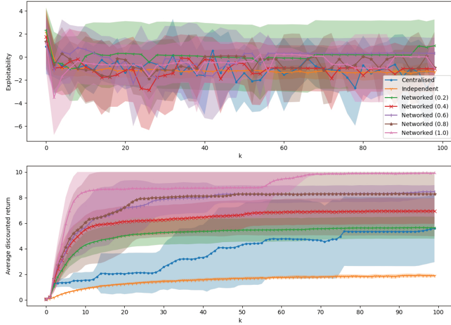
Fig. 2. ‘Cluster’, pop.-independent, 100x100 grid.
