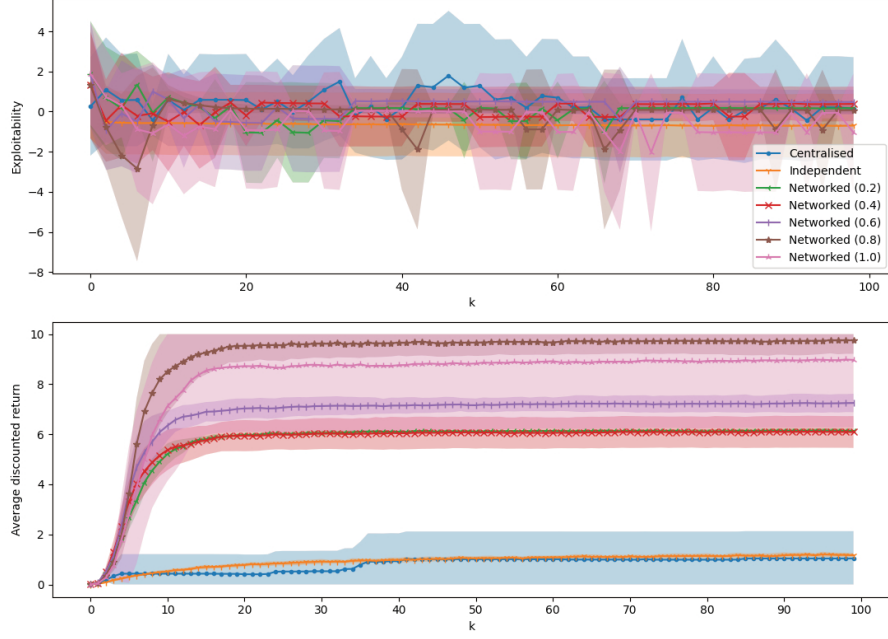
Fig. 1. ‘Target agreement’, pop.-independent, 100x100 grid.
