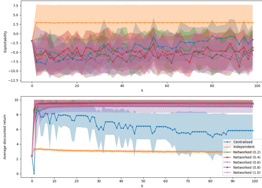
Fig. 5. ‘Disperse’ task, population-independent policies, 100x100 grid.
