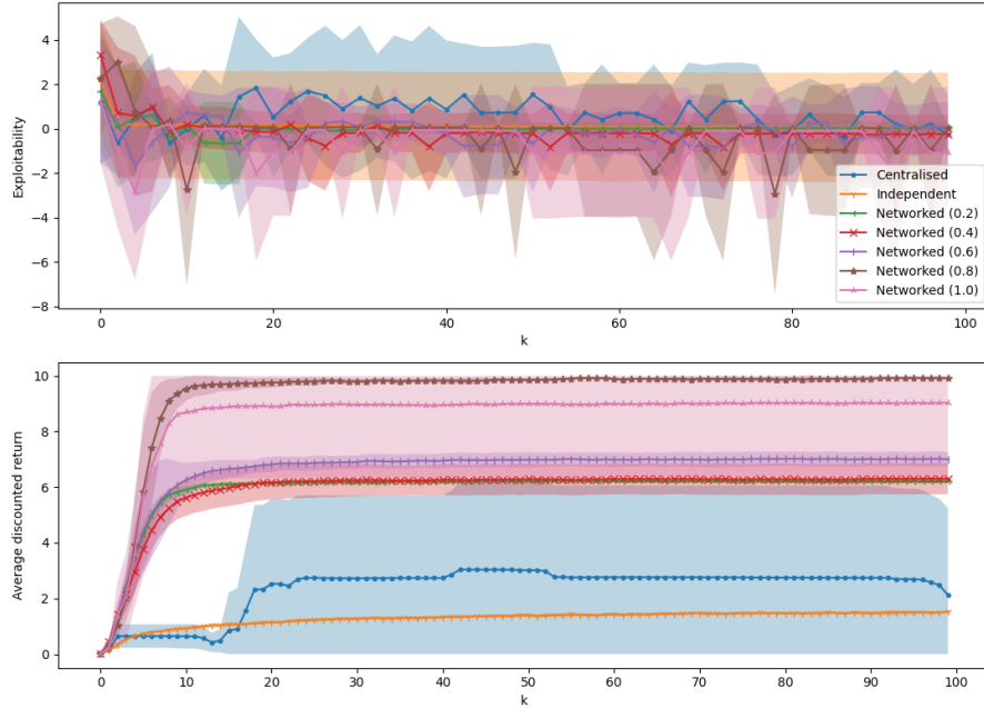
Fig. 3. ‘Target agreement’ task, population-independent policies, 50x50 grid.
