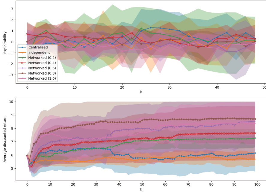
Fig. 8. ‘Push object’ task, population-dependent policies with global observability of mean field, 10x10 grid.
